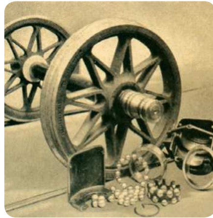
In 1911, for the first time, Swedish long distance passenger coaches had axleboxes incorporating two SKF double row self-aligning ball bearings
