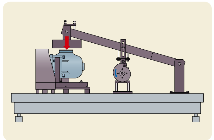
SKF V2F testing principle
