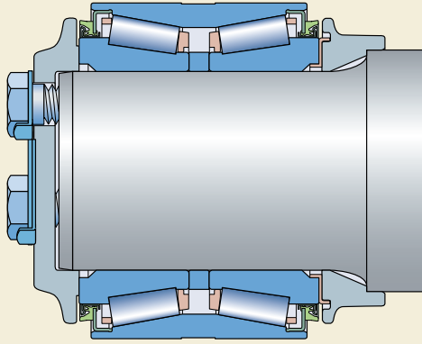
Metric size compact TBU for Chinese freight cars
