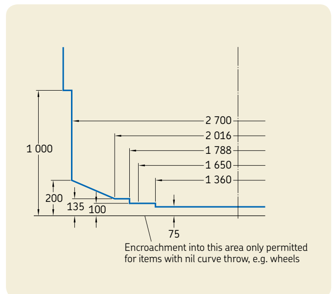
Example of British vehicle loading gauge
