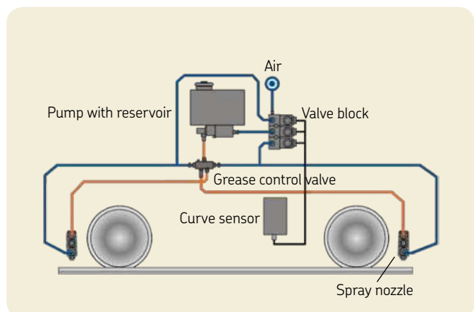
SKF EasyRail Track lubrication system
