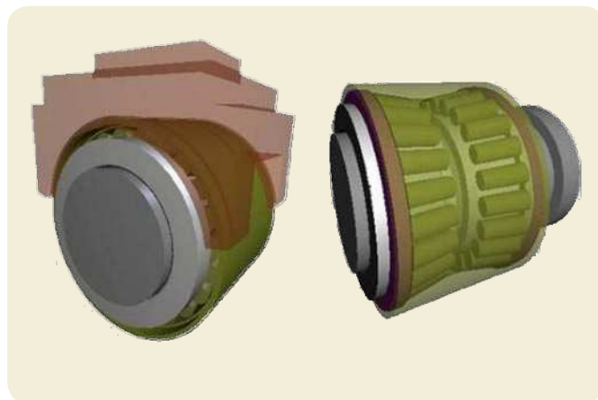
Model of a tapered roller bearing application with a saddle adapter
