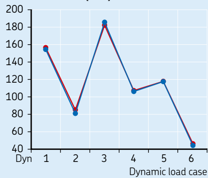
Strain gauge 5 von Mises stresses [MPa]
