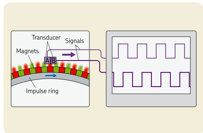
Rotational speed "Single head" SKF Axletronic sensor with two channels
