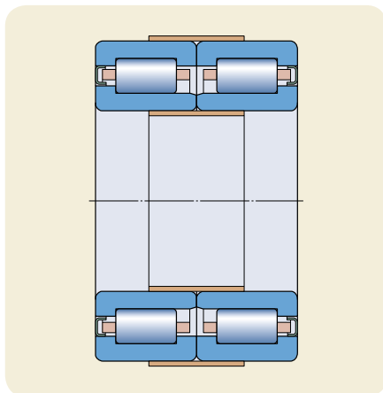
Short CRU design with a mounting sleeve on the inner rings and outer rings to facilitate mounting
