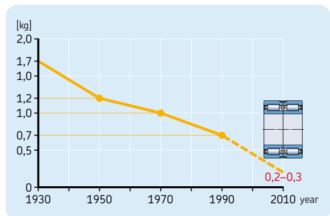
Grease quantity of a typical German freight car axlebox
