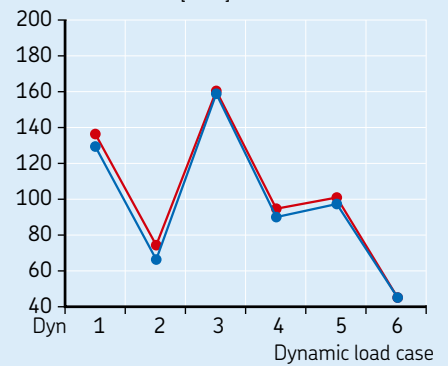
Strain gauge 6 von Mises stresses [MPa]
