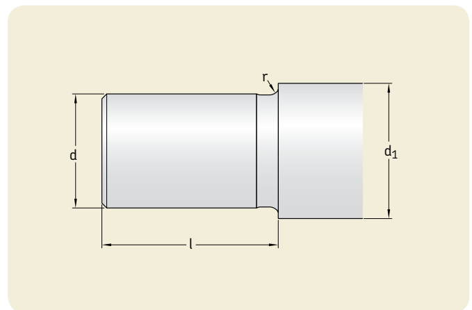
Principal dimensions of an axle journal
