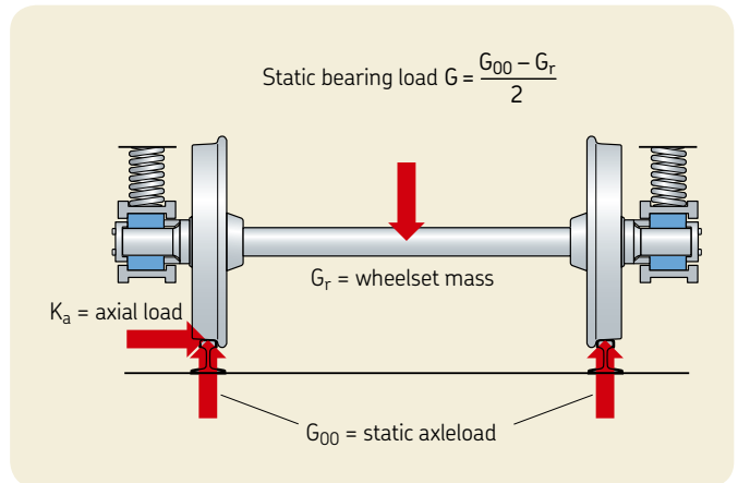
Acting bearing loads principles
