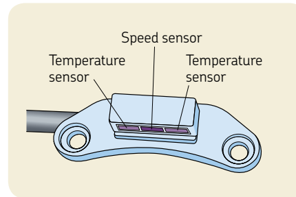
"Single head" SKF Axletronic sensor system
