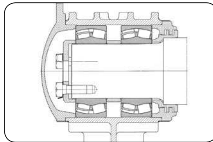
Bearing arrangement
