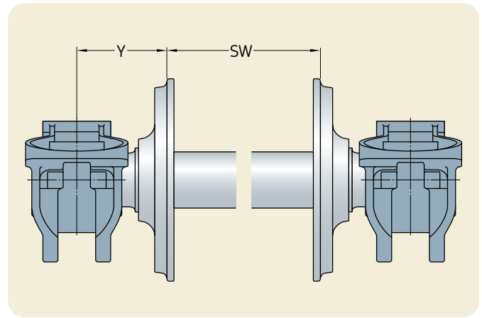
Principles of axial wheelset/axlebox distances
