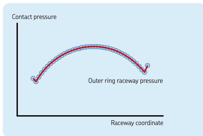
Contact pressure on the outer ring raceway for an adapter application
