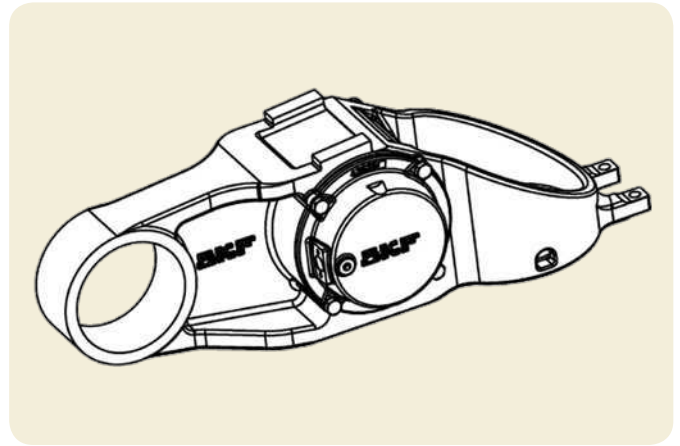
Typical one-piece link arm axlebox design
