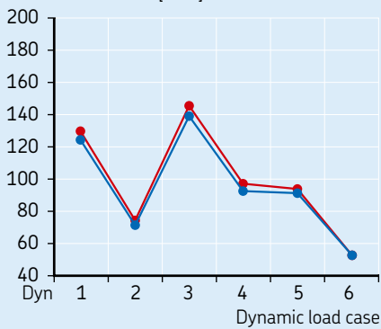
Strain gauge 3 von Mises stresses [MPa]
