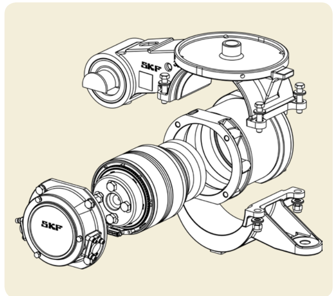
Typical three-piece link arm design
