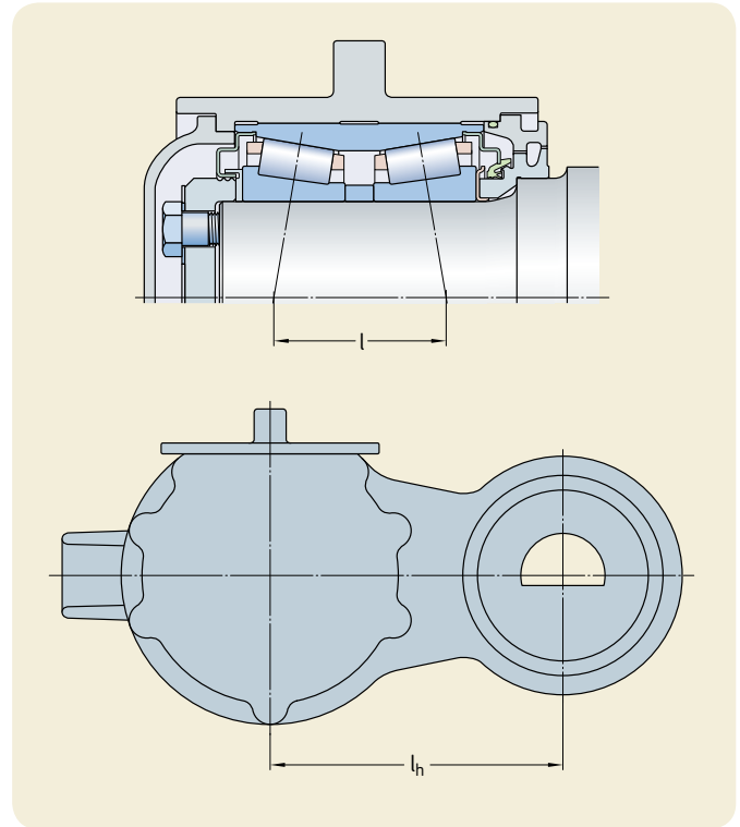
Link arm axlebox calculation model
