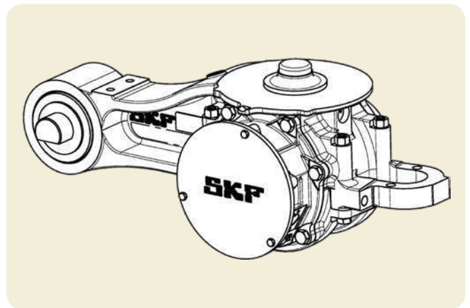
Typical two-piece link arm design
