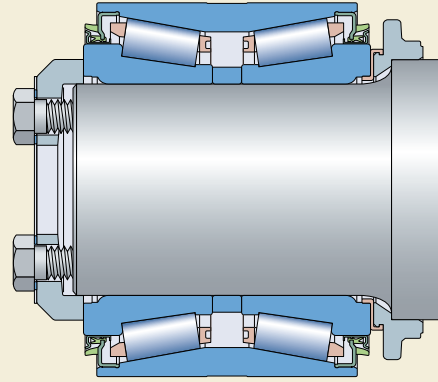
Compact TBU for Russian freight cars
