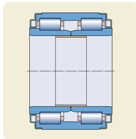
Long CRU design with a mounting sleeve on the inner rings
