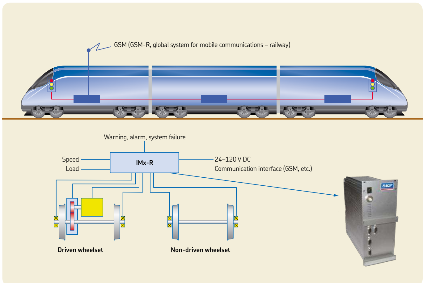
SKF Multilog online system IMx-R installation
