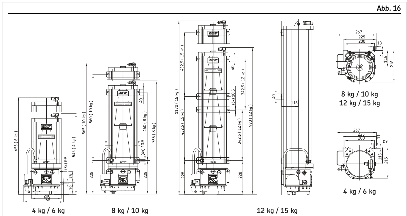
Abmessungen KFGL/KFGS in mm
