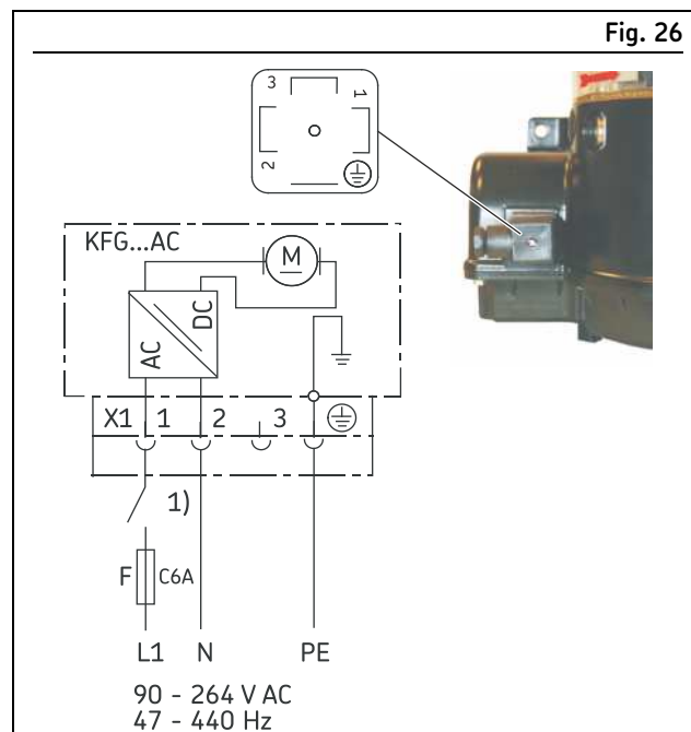
Connector pin assignment for 230 VAC (90-264 VAC)
