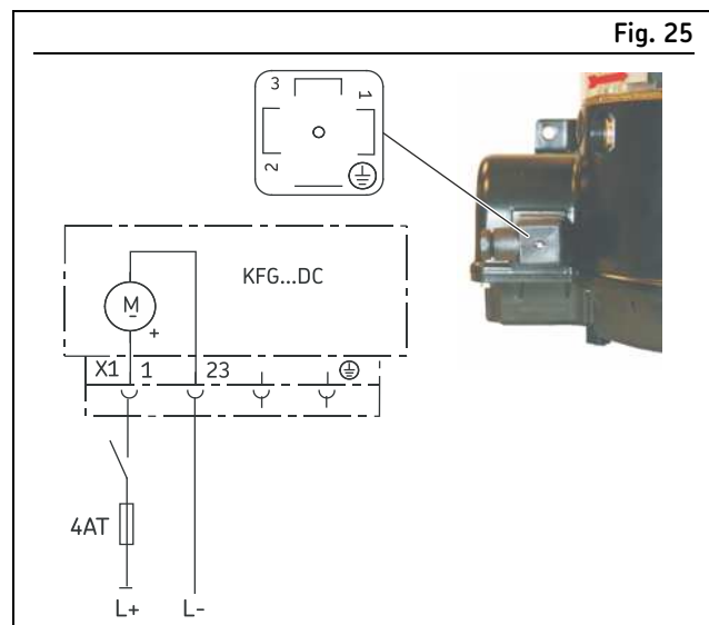
Connector pin assignment for 24 VDC
