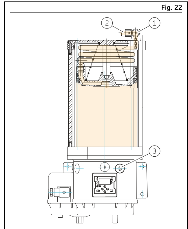
Fill connection on the reservoir cover
