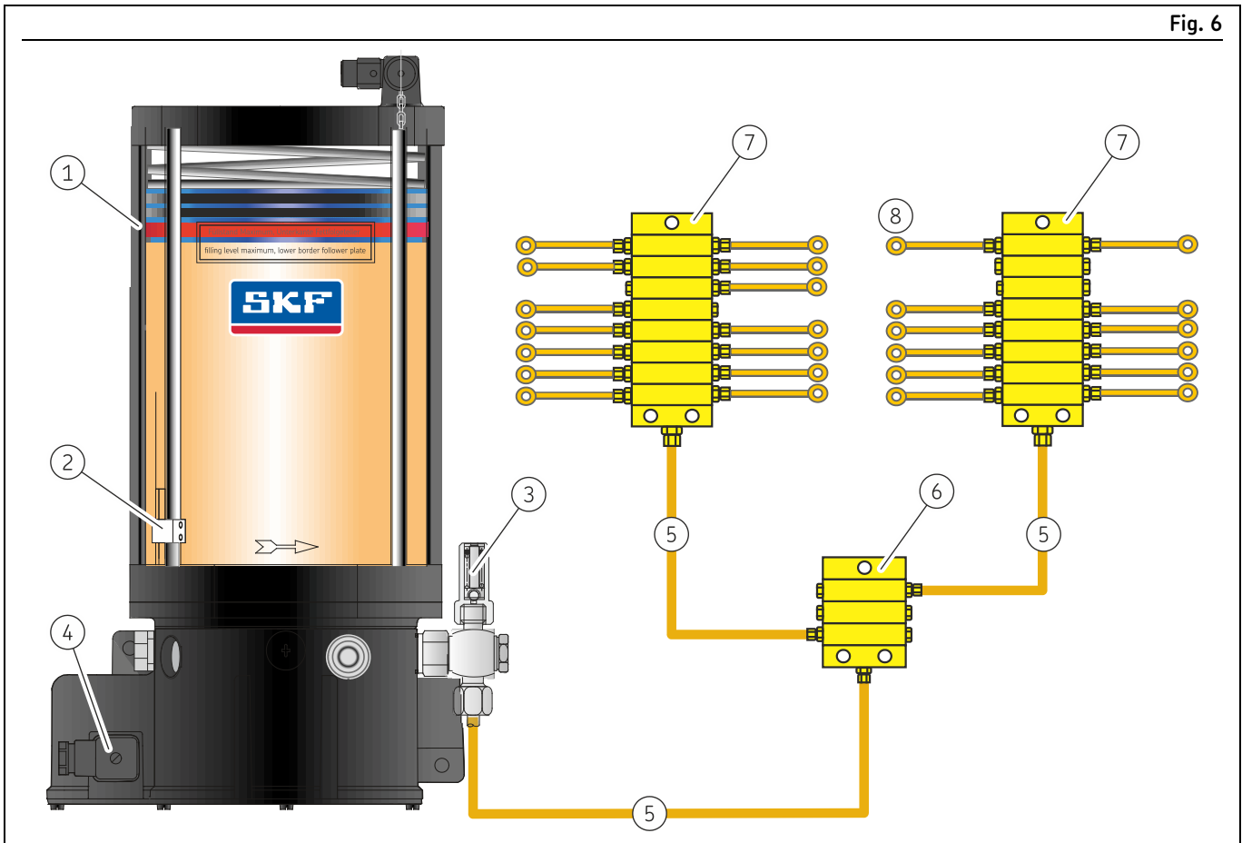
Progressive system with KFG pump unit
