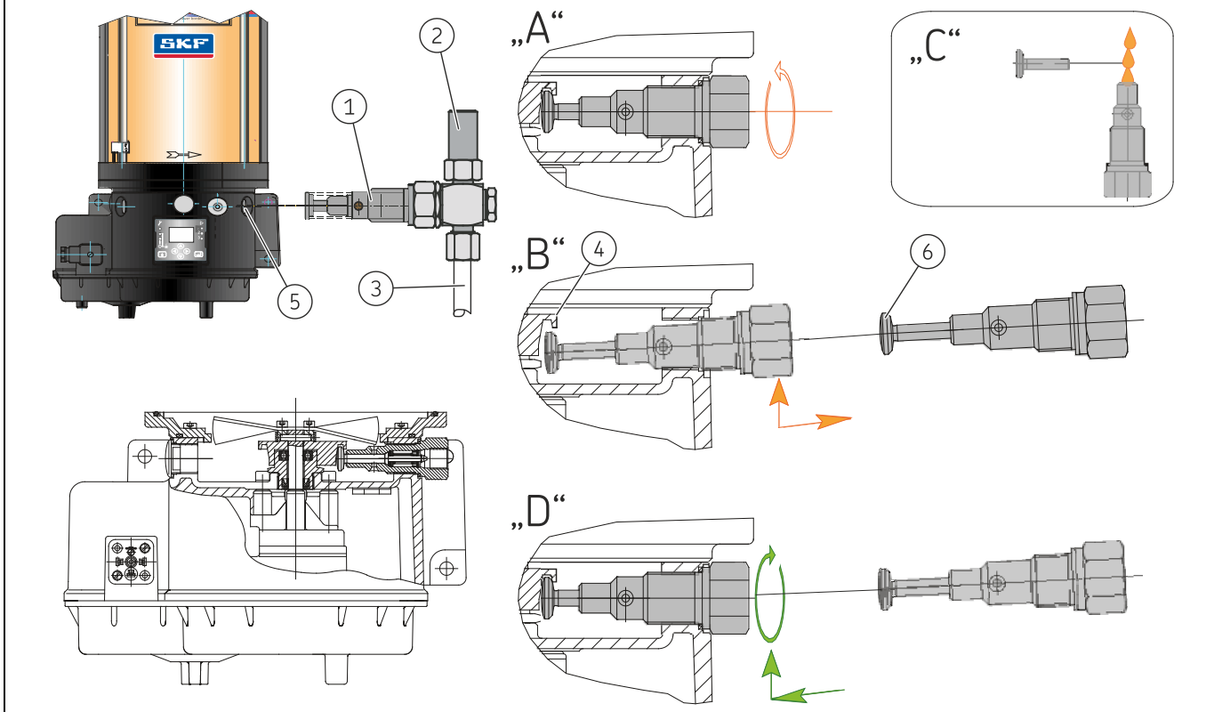
Installing a positively driven pump element
