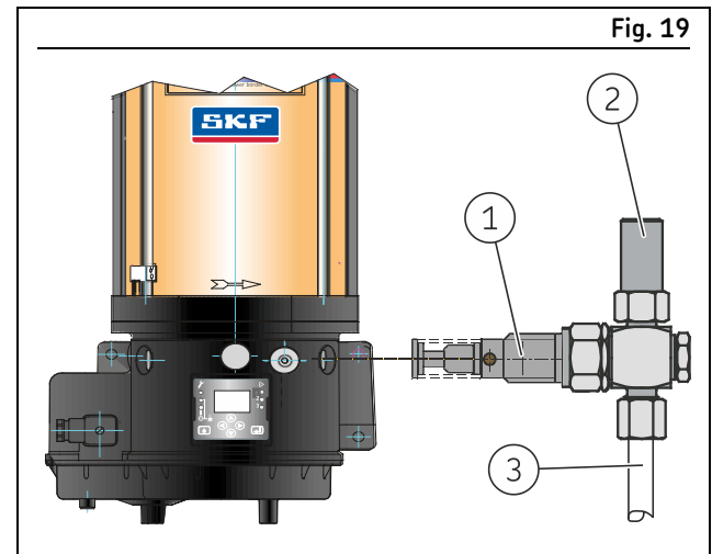
Installing a spring-return pump element
