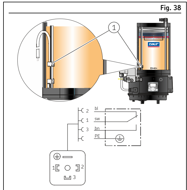
Lubricant level switch
