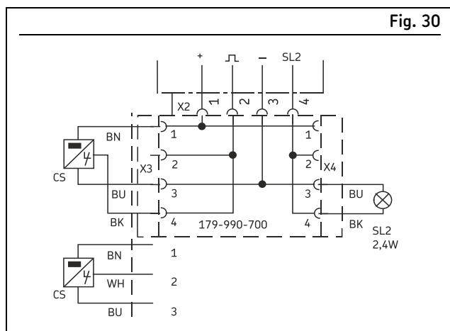
Connector pin assignment
