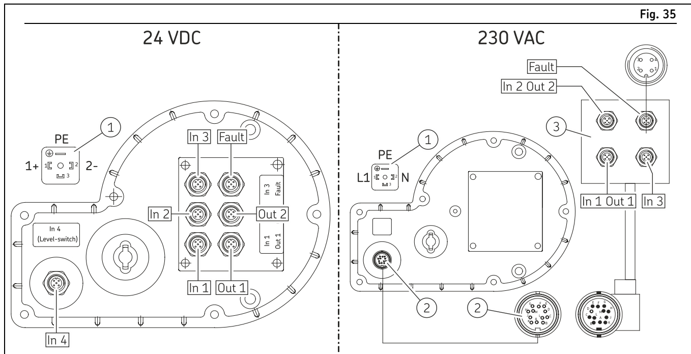
KFGL pump unit, ProFlex programming
