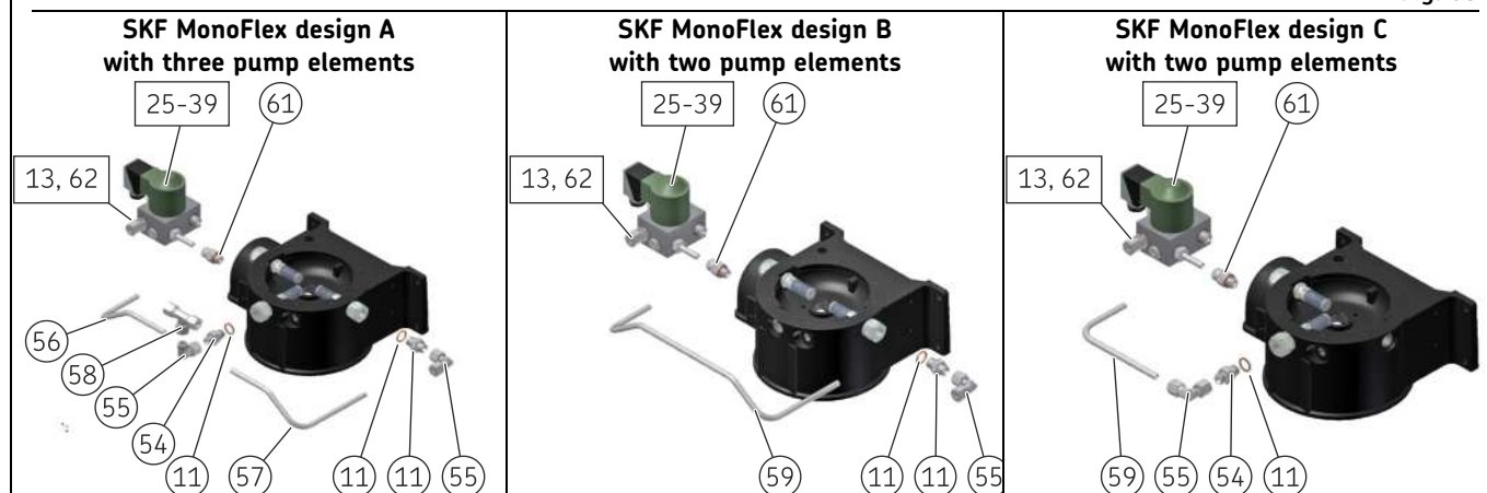
Exploded-view and spare parts drawings
