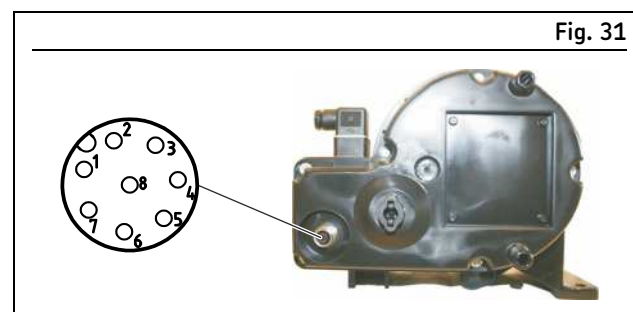
Plug-and-socket connection according to EN 60947-5-2
