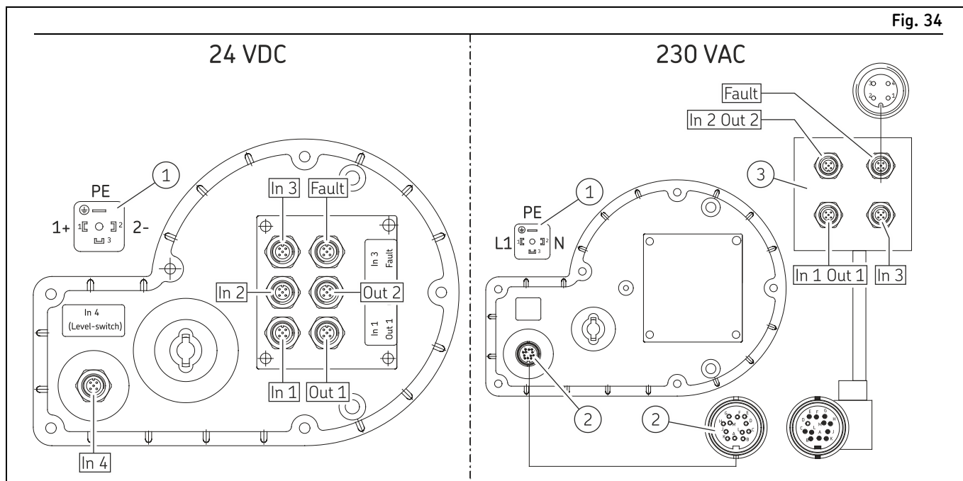
KFGL pump unit, MonoFlex programming
