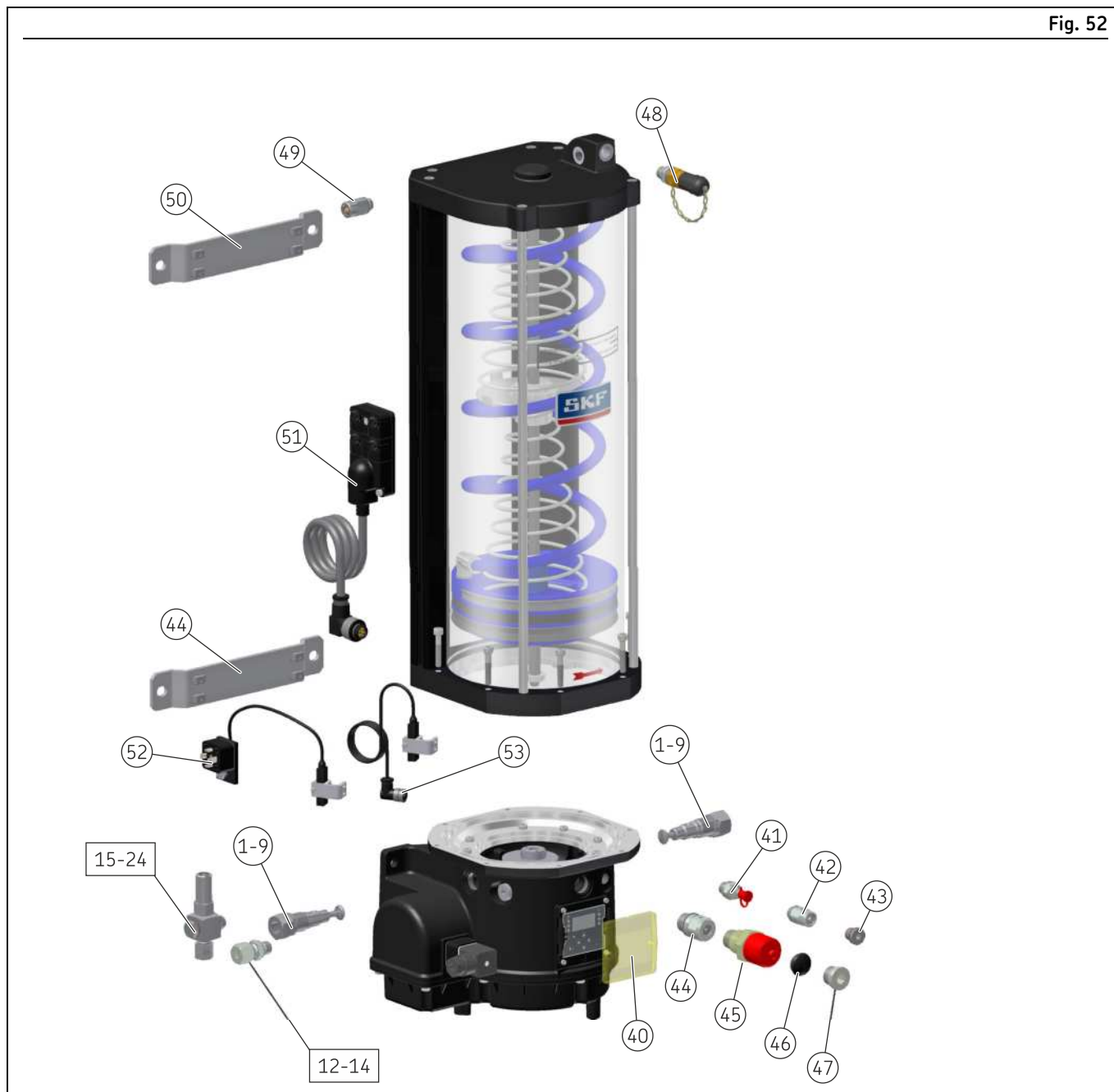
Exploded-view and spare parts drawings
