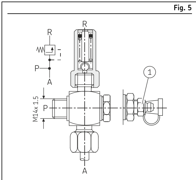
Pressure limiting valve
