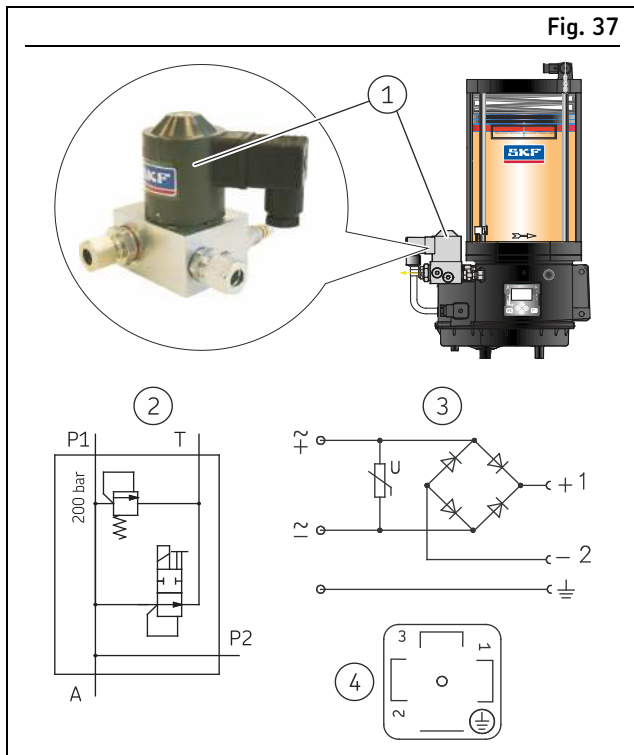
Pressure relief valve/pressure limiting valve
