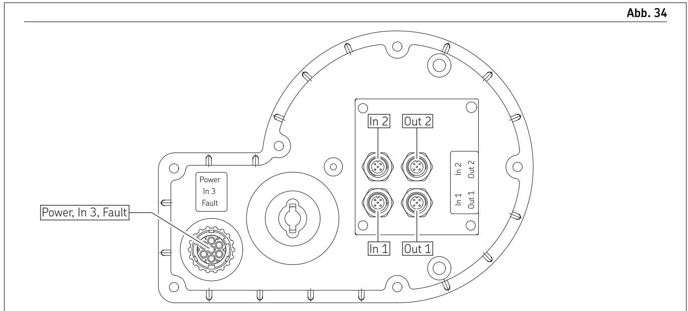
KFGL-Pumpaggregat, MonoFlex-Programmierung
