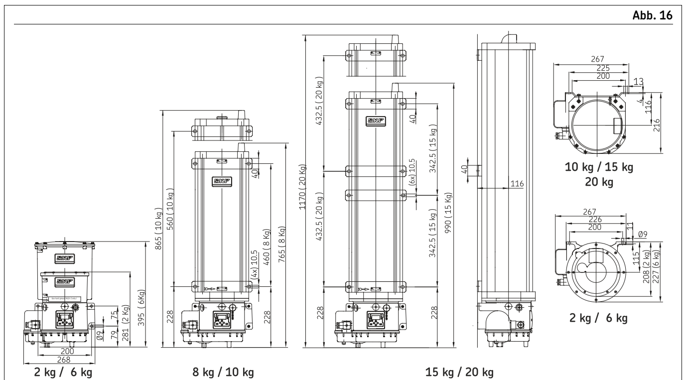
Abmessungen KFGL/KFGS in mm
