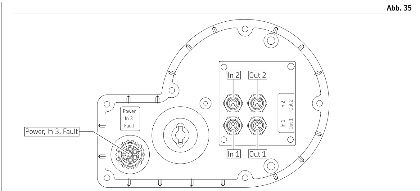
KFGL-Pumpaggregat, ProFlex-Programmierung
