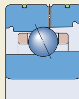
Open variant for direct oil lubrication
