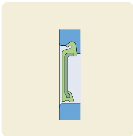
Non-contact seal for high-speed operation
