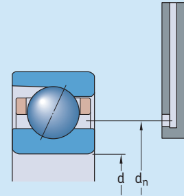
Oil nozzle position for oil-air lubrication
