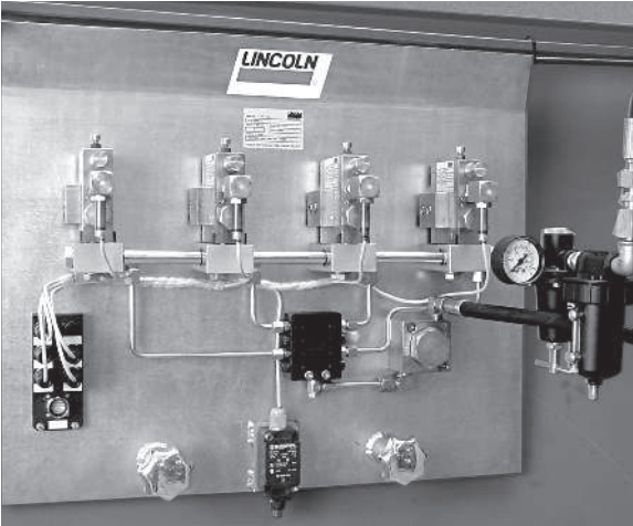
Bracket Mounting (Bracket 515-31225-1) of SDLH Nozzles
