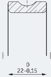
Fig. 3: Deep groove ball bearing inner ring width specification with default specification operator.
