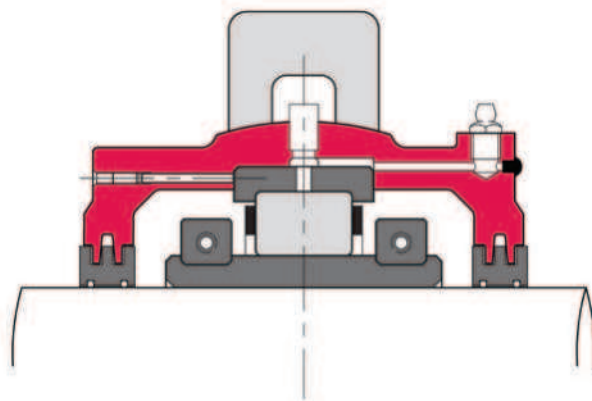
EXILOG BEARING
