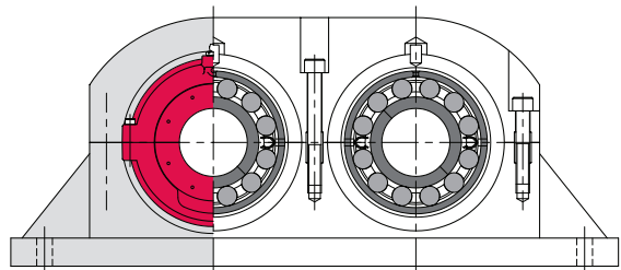
Custom double housing
