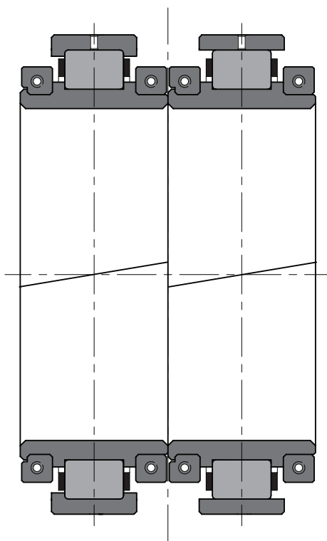
DOUBLE BEARING
