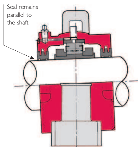
COOPER SPLIT ROLLER BEARING
