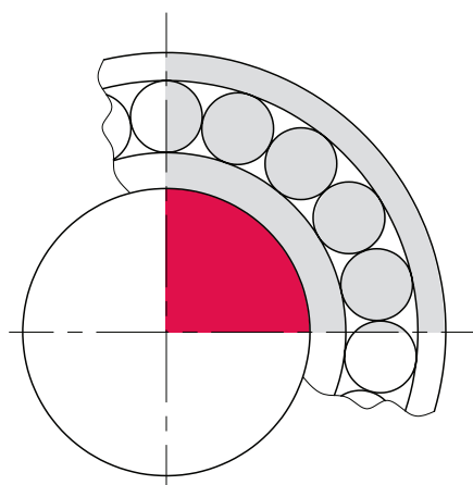
FULL ROW BEARING
