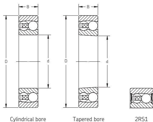
Cylindrical bore
