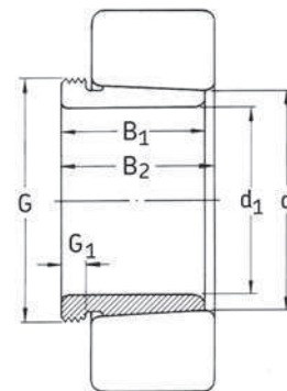
Type AH, AHX
