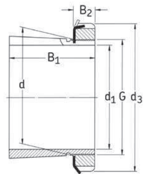
Type HA, HE
