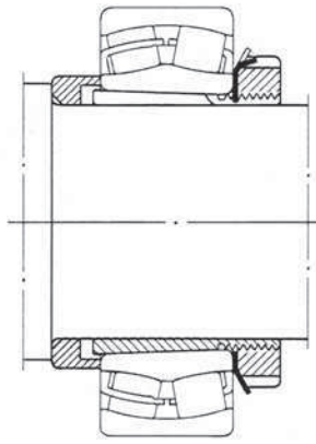
Shouldered shaft mounting with adapter sleeve
