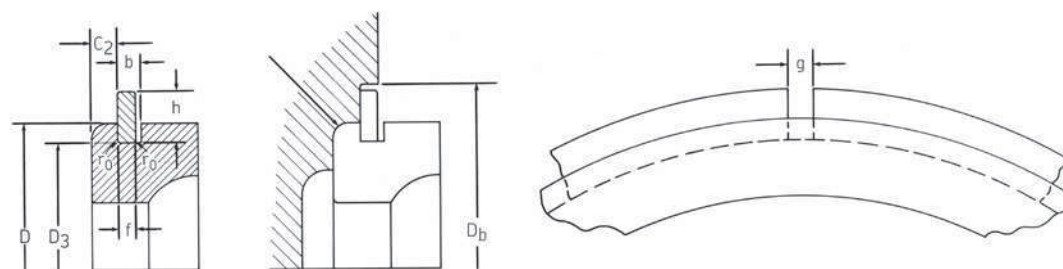
Snap ring and snap ring groove dimensions
