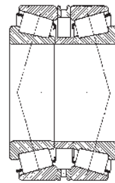
Back-to-back arrangement (Suffix DB)
