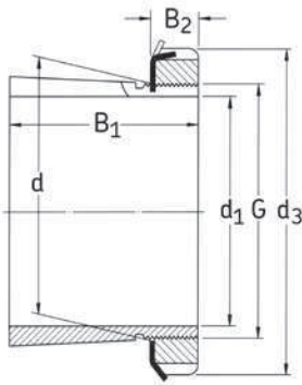
Type HA, HE
