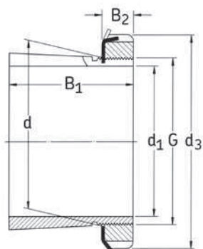
Type H MB locking device
