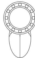
Figure C: Load distribution in a bearing with end play.
