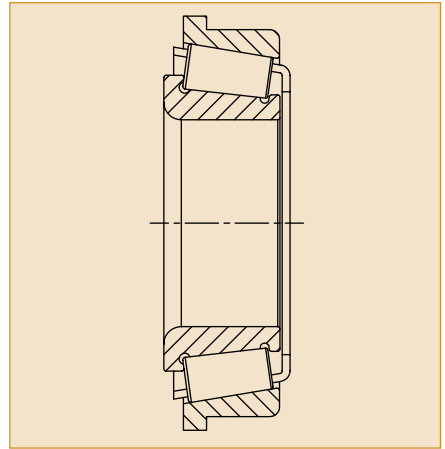
Flanged Cup
