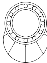
Figure B: Load distribution in a bearing with 0µm preload/0µm End Play.
