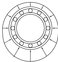
Figure A: Load distribution in a bearing with preload.
