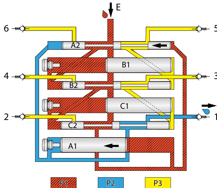
Fig. 17 Course of the lubricant illustrated by means of an SSSD-6 metering device phases 11 and 12
