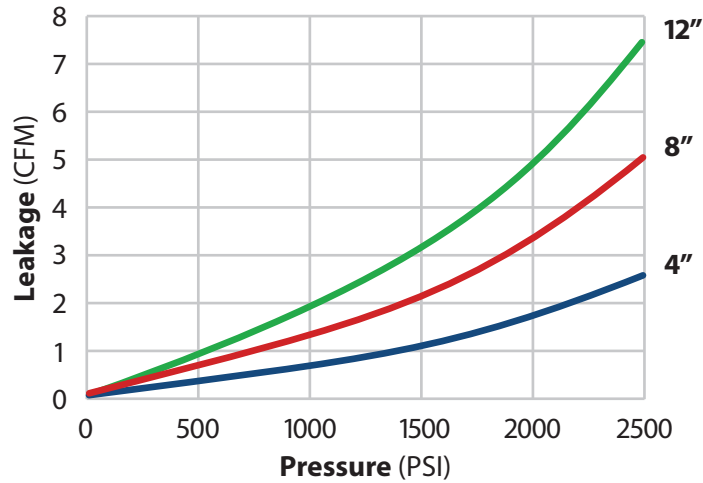
[K•DGS] Leakage rates (350 fps)
