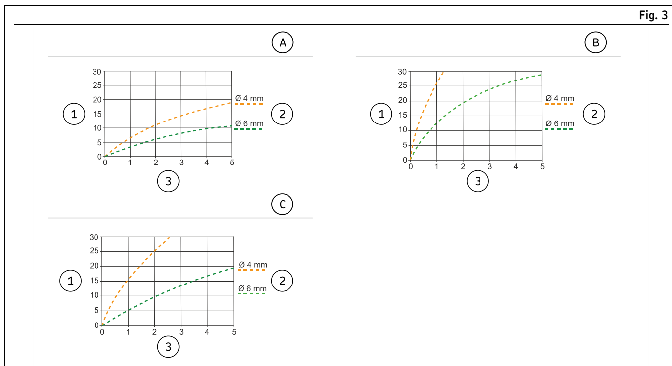
Delivery pressure as a function of line length, line diameter, and temperature
