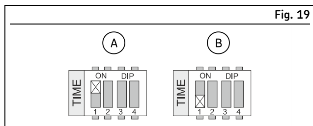
Activating/deactivating the TLMR
