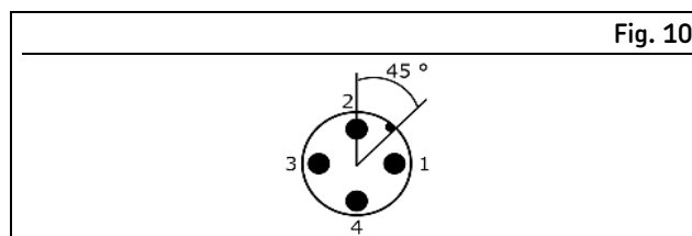
Pin assignment of M12 connector
