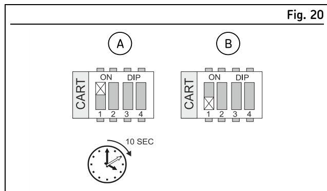
Carrying out a reset
