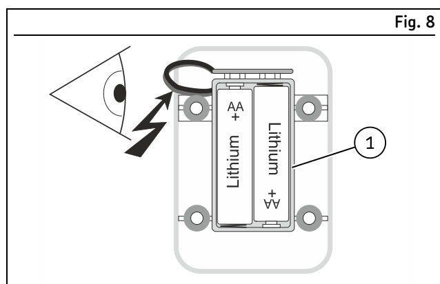
Checking the wires
