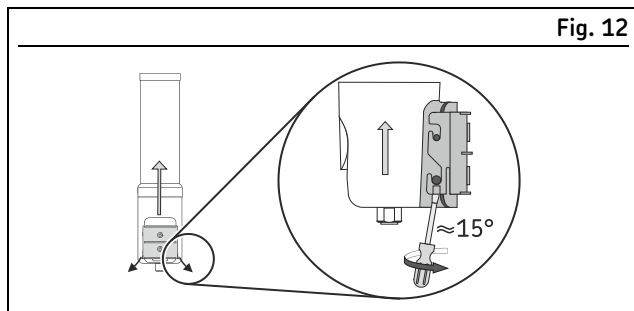
Removing the TLMR from its bracket
