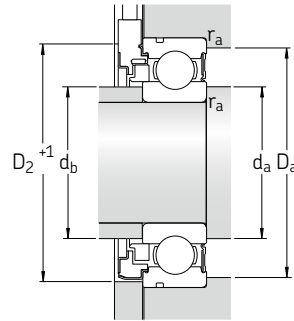
BMB BMO 端盖孔径 \geq D_2 + 1 \text{ mm}
