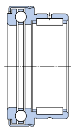
NKX..Z (F w ≥ 12 mm)
