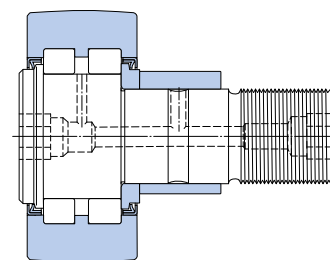
PWKR ...2RS
