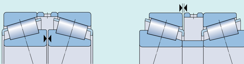
面对面或背对背配置的公制配对单列圆锥滚子轴承的轴向游隙
