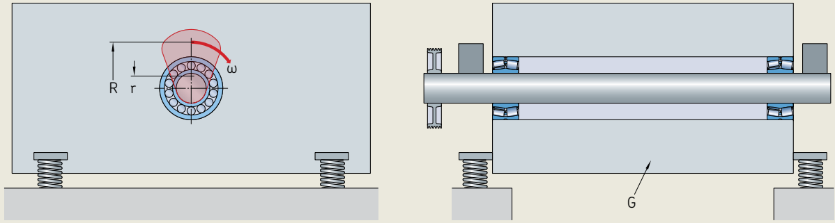
圆振动筛
