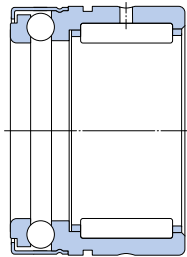
NX..Z (F w ≥ 10 mm)
