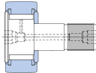
KRV..PPA ( 22 \leq D \leq 26 \text{ mm} )
