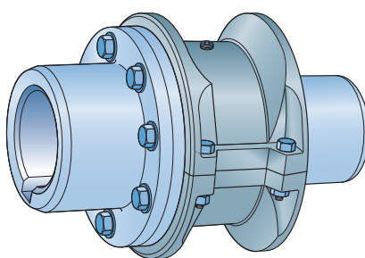
Half spacer
